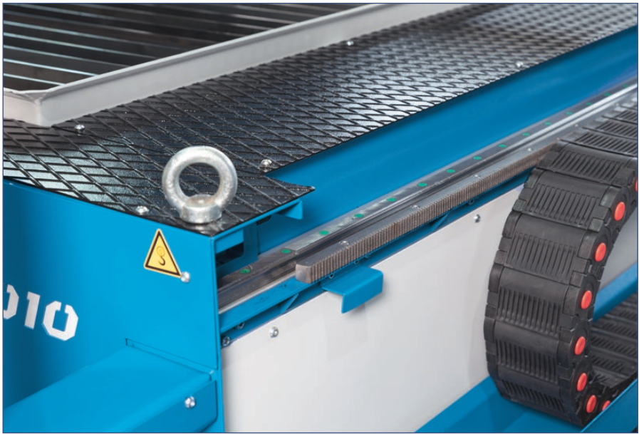
Low-wear and low-maintenance helical gears are designed for continuous operation
