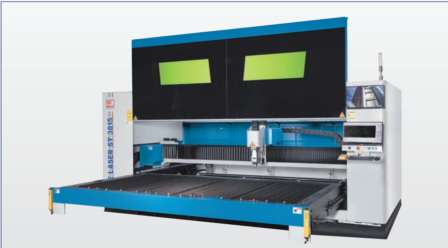
The work table is mounted on a heavy-duty pull-out mechanism and easily can hold loads up to 1000 kg in the fully extended position
