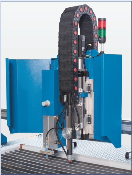
Quick-coupling at the cutter head reduces tooling time
