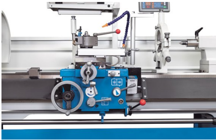
The slip coupling for the automatic feed is positioned centrally on the apron for easy adjustments
