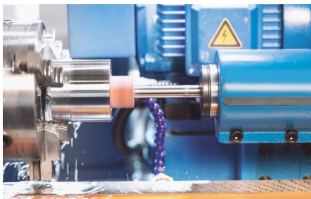
Allows inside grinding depths up to 4.9"
