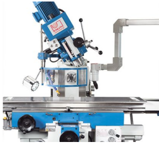
Cutter head swivels \pm 45^\circ
