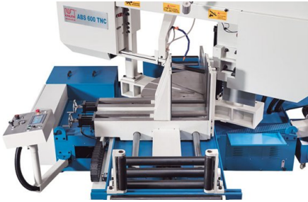
Manual saw frame angle adjustment with hydraulic drive (15°, 30° and 45°)
