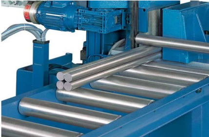
A bundle vise is provided for cutting entire material packs to length
