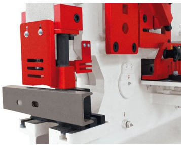
Notching station with safeguard
